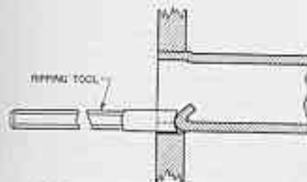
(3) USING A RIPPING TOOL TO CUT A SPLIT IN THE END OF A TUBE
